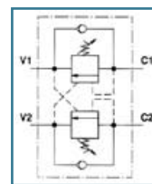
Hydraulic circuit plan
