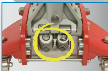
double pump system for faster lifting
