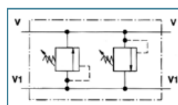
830 775 + 830 785 Hydraulic circuit plan
