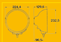
High beam headlight Luminator with parking light
