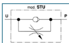
830 855 + 830 865 Hydraulic circuit plan
