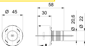
WEO K07 VCO
