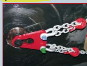
Anchor shackles (code-no. 551 185, see page 207) (2 pieces necessary) further shackles
