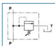
830 745 Hydraulic circuit plan
