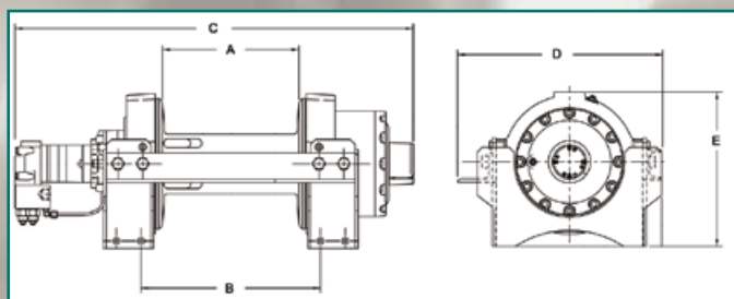
picture shows RPH 30000 with optional rope tensioner.
