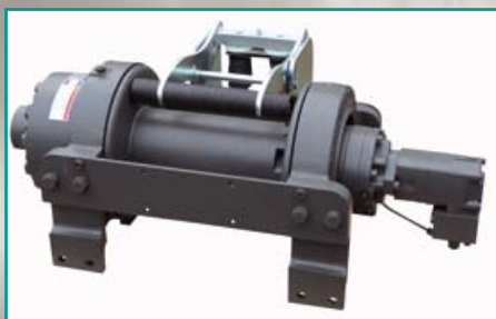
picture shows RPH 30000 with optional rope tensioner.
